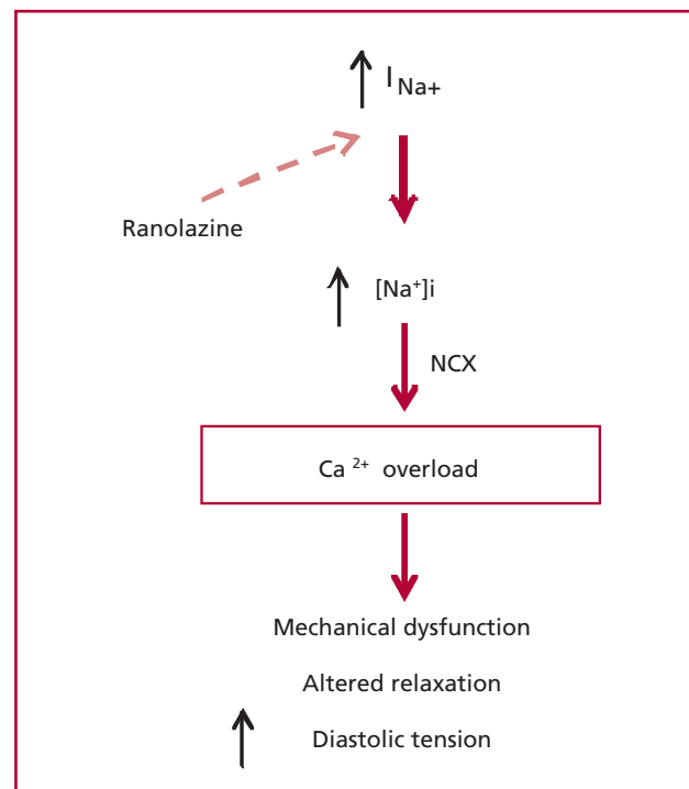
Fig. 1. Increased \text{Na}^+ current ( I_{\text{Na}^+} ) leads to higher intracellular \text{Na}^+ concentration ( [\text{Na}^+]_i ). These changes lead to \text{Na}^+/\text{Ca}^{2+} exchanger (NCX) activity with concomitant \text{Ca}^{2+} overload, which would be responsible for diastolic dysfunction. Ranolazine by inhibiting I_{\text{Na}^+} current would attenuate mechanical dysfunction.
