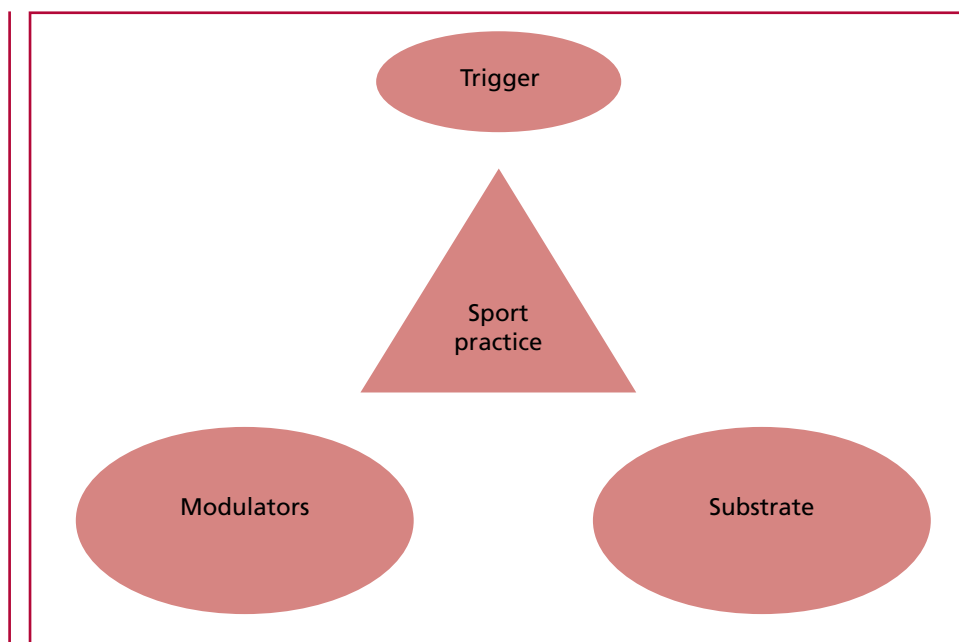
Fig. 1. Coumel's triangle
