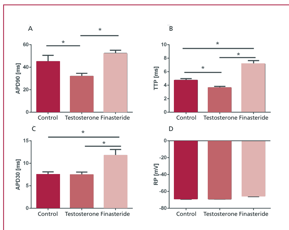
Fig. 1. Changes in action potential parameters in the rat right ventricle. APD90: action potential duration at 90% repolarization; APD30: action potential duration at 30% repolarization; TTP: time to peak; RP: resting membrane potential. * = p < 0.05 ; n = 5 ).
