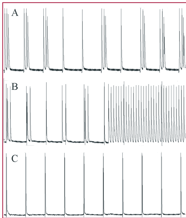
Fig. 2. Action potential recordings following terfenadine and pinacidil treatment and the arrhythmia protocol. Panels A , B and C show representative action potentials following application of the arrhythmia protocol (10 Hz for 10 seconds, 20 Hz for 10 seconds and 0.5 Hz for 1 minute) in the isolated right ventricle, perfused with Tyrode solution supplemented with terfenadine and pinacidil, of control rats ( A ), rats treated with testosterone ( B ) and rats treated with finasteride ( C ).
